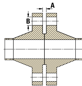
Flange Dimensions
